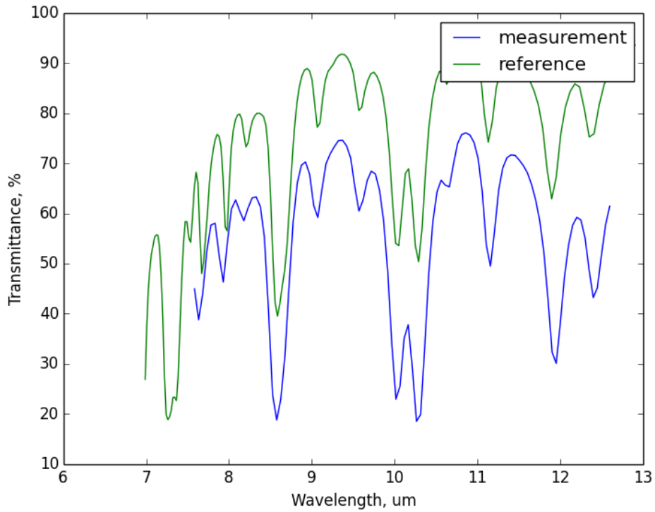
Figure 4: Transmission spectrum measured by the Owl compared to a reference measurement. Matching the absorption features (troughs) identifies any shift in the wavelength response.
