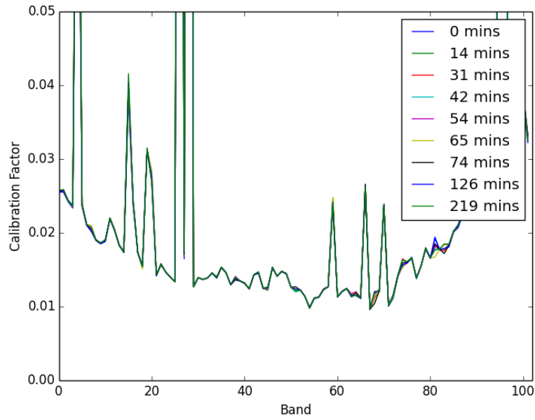
Figure 3: Calibration data for a single spatial pixel after various time delays.
