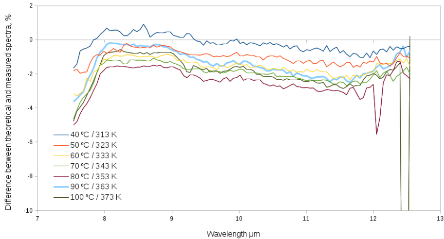
Figure 5: Percentage spectral error at different target temperatures. Some of the error may be due to inaccuracy in the target black body temperature.
