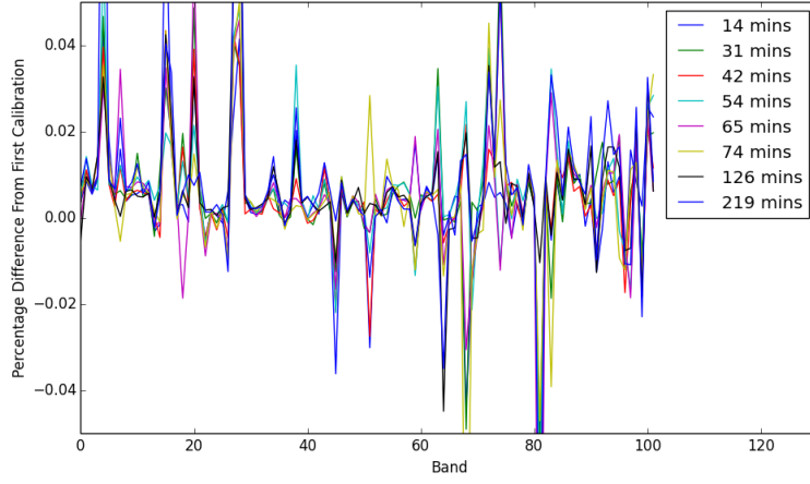
Figure 2: Percentage difference in each of the calibration files from the first calibration file for a single spatial pixel.
